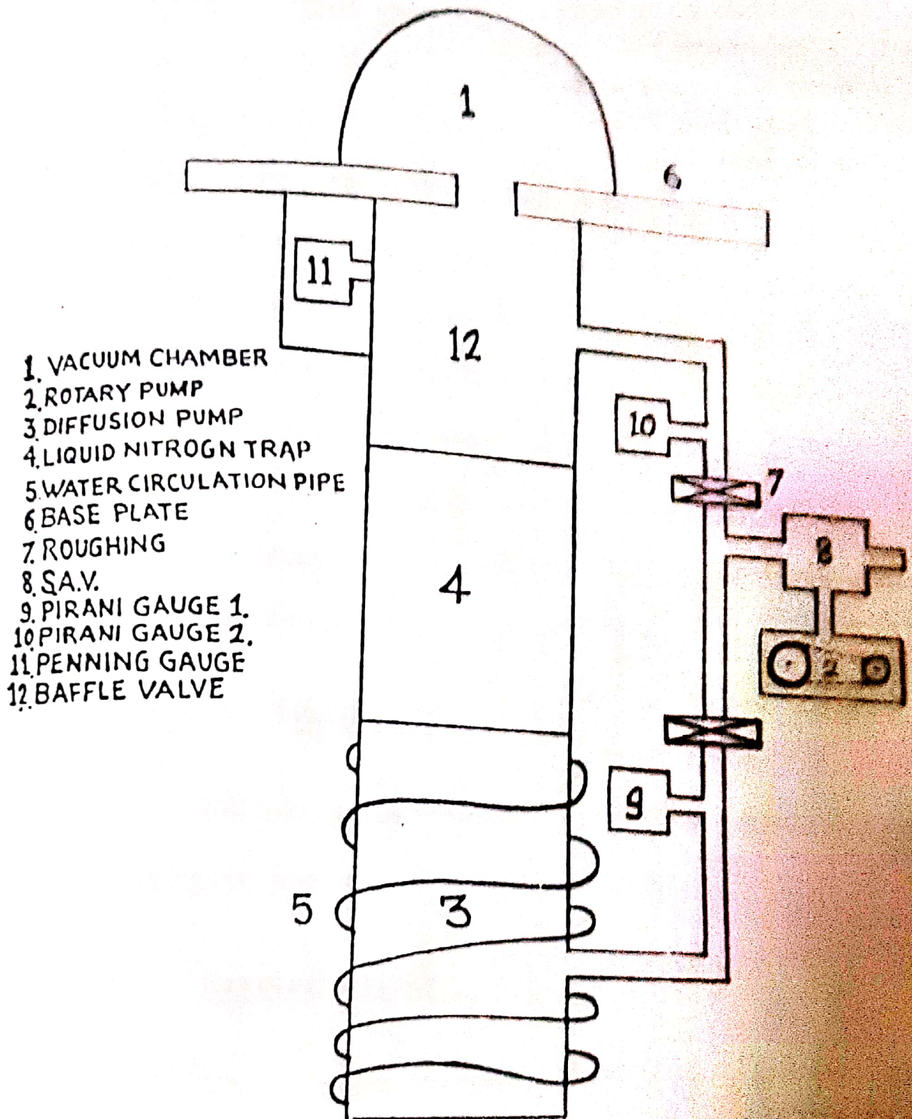
SKETCH DIAGRAM OF VACUUM COATING UNIT FIG. (4)
